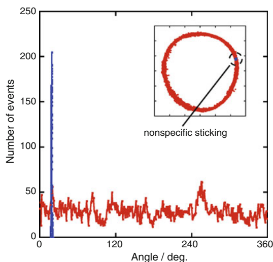
Fig. 3 Measurement error of image processing. Histogram of angle distributions of forcibly rotated (red) and fixed beads (blue) recorded at 1,000 frames/s. For this figure, the bead was forcibly rotated at constant rate (0.2 revolutions/s) using magnetic tweezers. The bead was nonspecifically fixed onto the glass by infusing buffer containing 100 \mu M \text{CuCl}_2 . Inset shows the trace of the centroid of bead images
